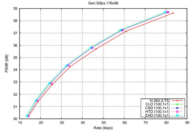
Fig. 2. Rate-distortion curves comparing the standard H.264/AVC encoder and the proposed technique ( 1 \times 1 ) for sequence Ger .
