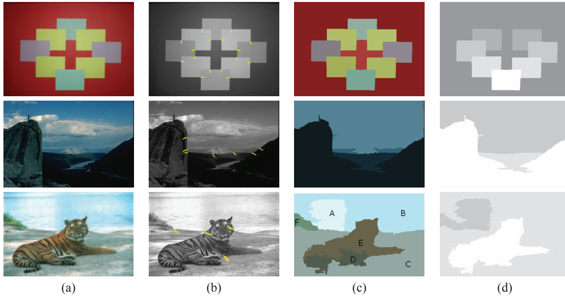
Fig. 4. Example of depth segregation. (a) Original image (b) T-junction detection (c) Segmentation (d) Depth ordering
