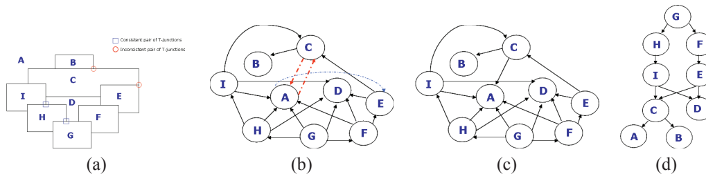
Fig. 3. (a) Partitioned image (b) Associated DG (c) Associated DAG (d) Hasse diagram resulting from the transitive reduction of the DAG
