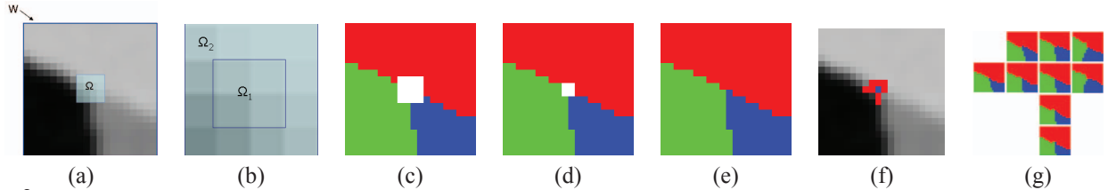
Fig. 2. (a) A window W centered at a candidate point: \Omega is the neighborhood we consider unreliable. (b) Partitioning of \Omega = \Omega_1 \cup \Omega_2 . (c) Branch extraction in W - \Omega . (d) Branch propagation in \Omega_2 . (e) Branch propagation in \Omega_1 . (f) Validated points: The point having the smallest value of sum of average curvature on each branch is marked in blue. (g) Cluster reduction.
