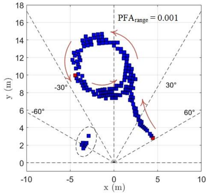
Figure 4. The graph shows a motorcycle occupying the center of the scene and doing some laps in front of the radar at an approximately constant speed.
