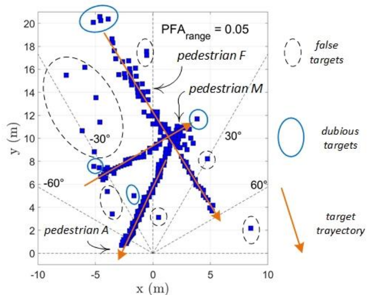
Figure 2. Global map of the received echoes along the time in scenario 1, while three pedestrians are walking along straight paths.
