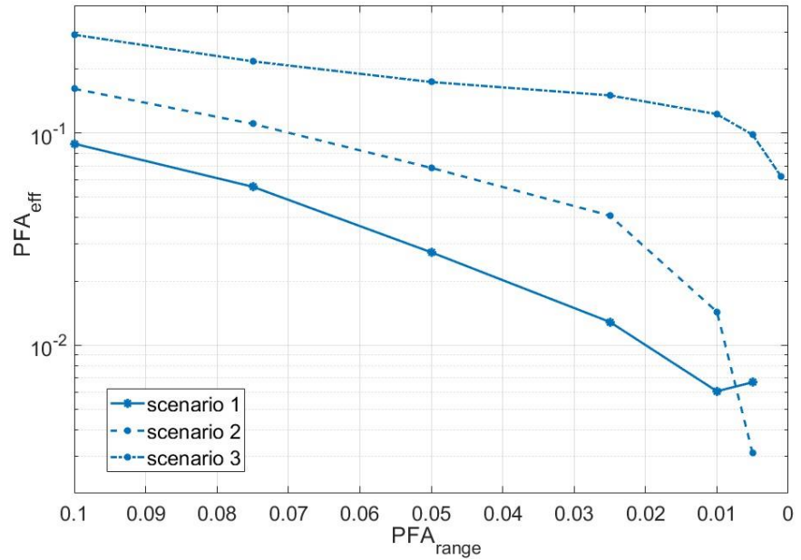
Figure 5. Effective probability of false alarm in the three scenes, obtained as a function of the PFA parameter chosen for the detection of targets in distance. For the selection of velocities, the value PFA_{vel} = 0.2 was used in all cases.
