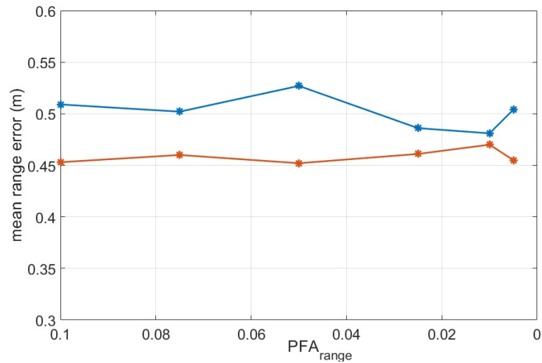
Figure 8. Mean range error obtained in the localization of the motorbike in scenario 2 along the two different paths.
