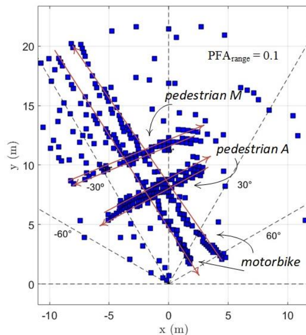
Figure 3. Echoes received over time in the second experiment, with two pedestrians going and coming along approximately the same path, and a motorcycle, describing the longest and most vertical paths.
