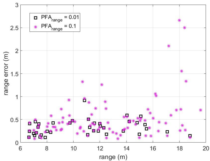
Figure 7. Range error committed along the tracking of one of the targets in scenario 1, for two values of the PFA_{range} parameter.
