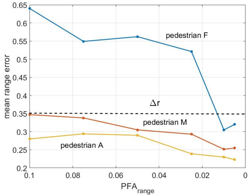
Figure 6. Mean error in distance obtained for individual targets in the first scenario
