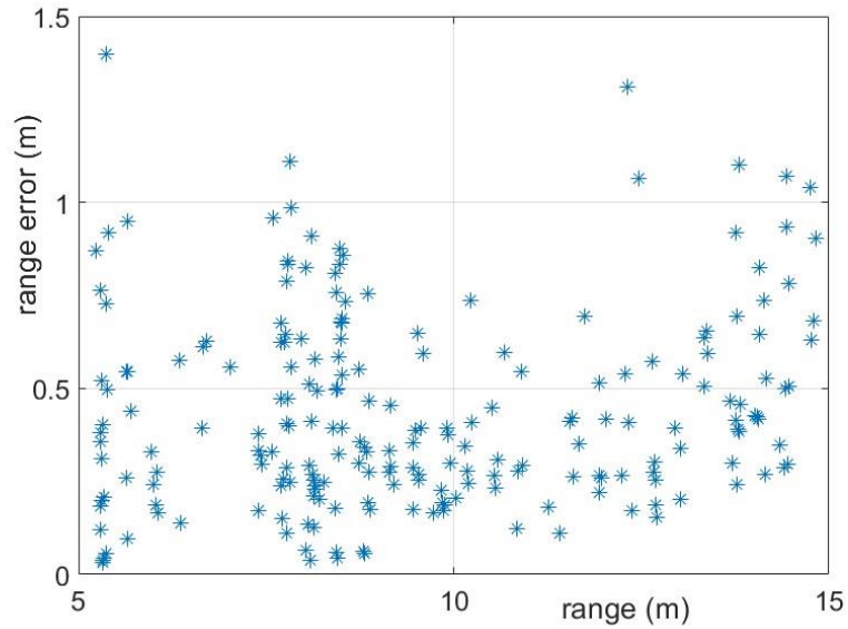
Figure 9. Estimated range error of the motorcycle in scenario 3, as a function of the distance to the radar, with PFA_{range} = 0.001 .
