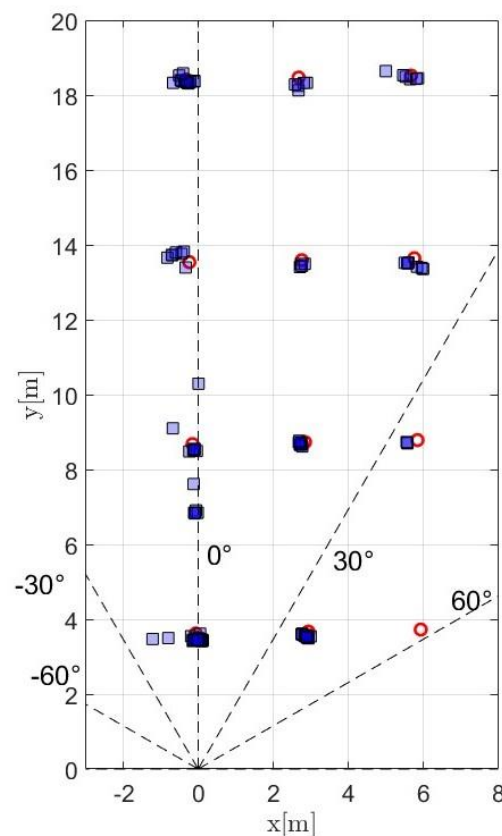
Figure 1. Measurements of a turning reflector on the calibration grid points.
