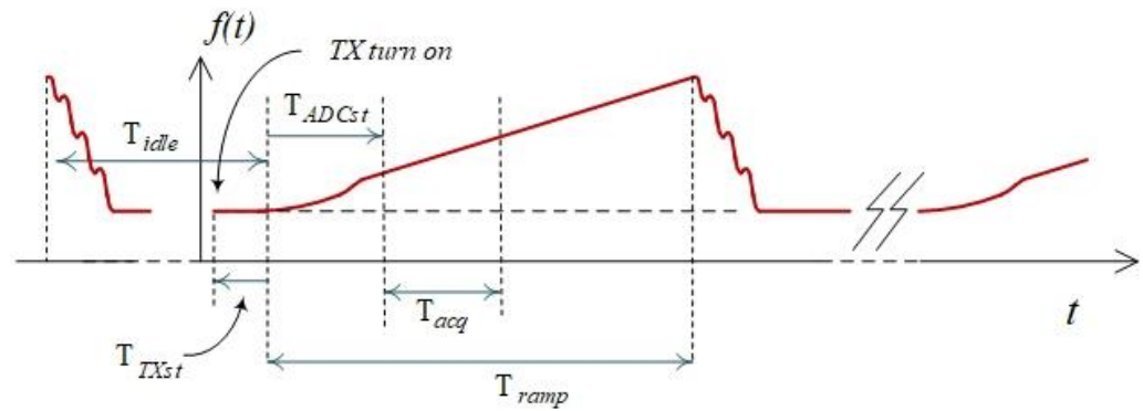
Figure 11. Signal time parameters in the radar configuration
